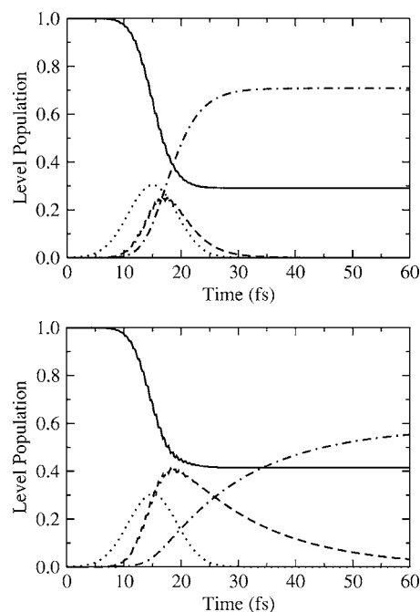
FIG. 2. Electronic level population after a 10 fs (FWHM) laser pulse excitation. Upper panel: the DTB–Pe–COOH system (for parameters see Table I), lower panel: the DTB–Pe–(CH 2 ) 2 –COOH system (for parameters see Table II), solid line: ground-state population P_g of the dye, dashed line: excited-state population P_e of the dye, dashed-dotted line: population P_{\text{ion}} of the ionized dye (what equals the total conduction band population), and dotted line: laser-pulse envelope (in a.u.).
